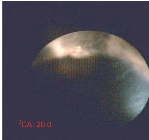
Fig. 3b. Photograph of the further development of the flame for 20 deg CA after TDC. The flame spreads over the whole combustion chamber and the flame front moves towards the zone of expression
