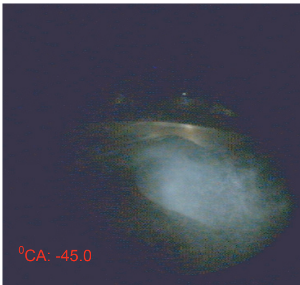
Fig. 2c. Photograph of injected fuel jet for 45 deg CA before TDC. Rebounding of the injected fuel jet from the piston head takes place
