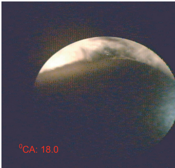
Fig. 3a. Moment of ignition took place for 10 deg CA before TDC. The photograph present the initial phase of flame development for 18 deg CA after TDC. High whirling occurring in the combustion chamber is clearly visible. This may be concluded from the character of the flame
